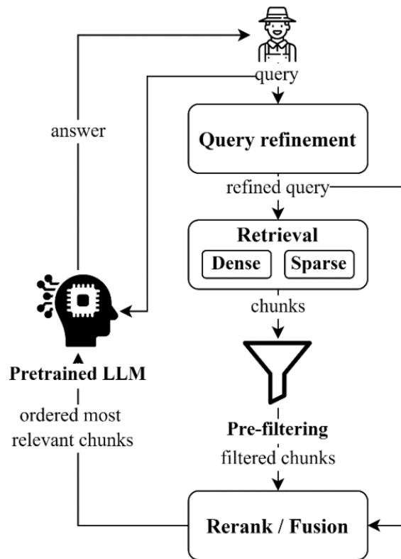
Gambar II.2 Inference Pipeline RAG modular berdasarkan taksonomi (Vizniuk2024).
