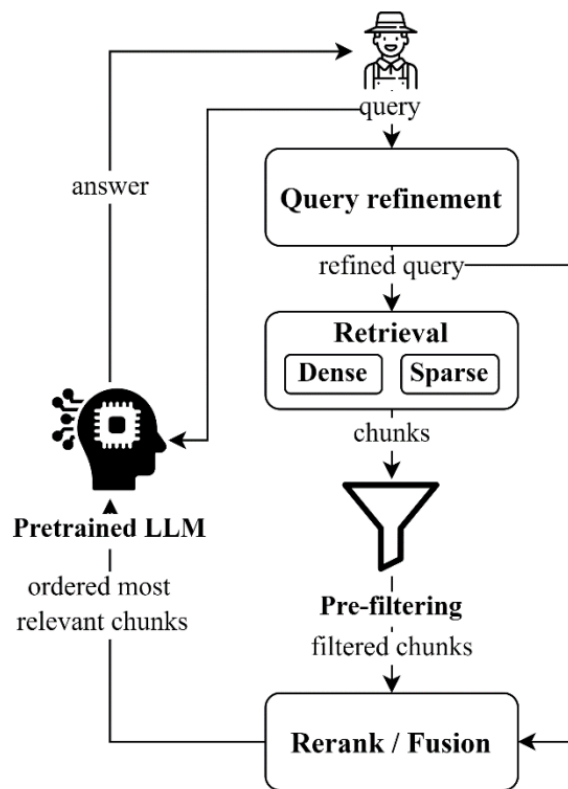
Gambar II.3 Inference Pipeline RAG modular berdasarkan taksonomi (Vizniuk dkk. 2024).
