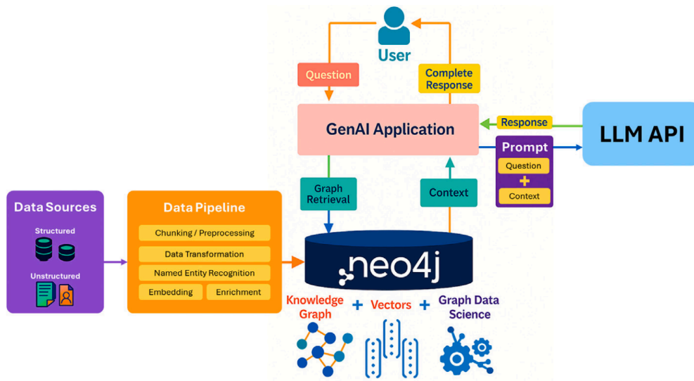
Gambar II.5 Gambaran umum pipeline Graph-RAG (Kamalipour, Asadi, dan Chimeh 2026)
