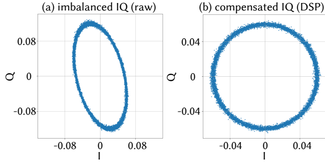
Fig. 4. IQ imbalance compensation using a 1 ms capture. Quadrature demodulation involves mixing received RF signal with local oscillator signals in the orthogonal I and Q channels. Mismatch in phase or amplitude between these channels manifests as an imbalance in the supposedly orthogonal IQ data (sin and cos). (a) amplitude imbalance in IQ resulting in an axis-aligned ellipse and phase imbalance causing tilt, along with DC offset causing an ellipse with a nonzero center. (b) blind IQ compensation [Windisch and Fettweis 2004] correcting for offset, gain and phase imbalances in our calibration pipeline. Notice the change in axis limits between (a) and (b); the reduced range in (b) reflects Q-channel gain correction normalizing to the lower I-channel amplitude.
