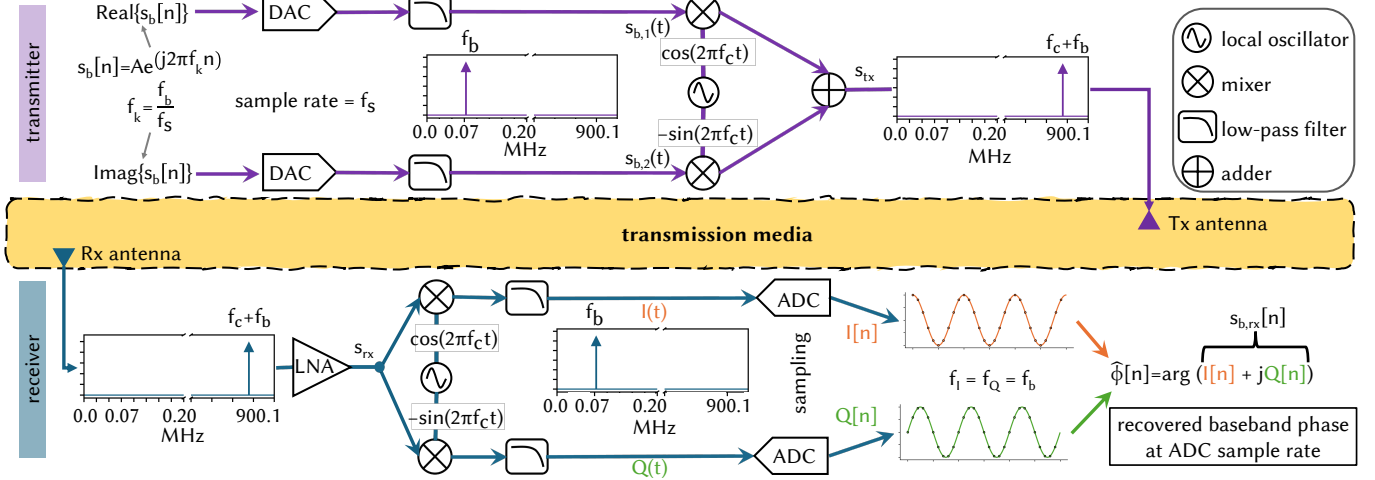
Fig. 2. Quadrature amplitude modulation and demodulation in an SDR transceiver. At the transmitter (top), a discrete-time complex baseband signal s_b[n] = Ae^{j2\pi f_k n} is generated, where f_b denotes the baseband frequency, f_s is the sampling rate, and f_k = f_b/f_s is the corresponding normalized digital frequency. The real ( \text{Real}\{s_b[n]\} ) and imaginary ( \text{Imag}\{s_b[n]\} ) components of the complex sinusoid are applied to separate digital-to-analog converters (DAC) and mixed with a common local oscillator at carrier frequency f_c \approx 900 MHz using \cos(2\pi f_c t) and -\sin(2\pi f_c t) , respectively. The mixer outputs are summed to form a real RF passband signal centered at f_{tx} = f_c + f_b , which is transmitted through the channel. At the receiver (bottom), the incoming RF signal is first passed through a low-noise amplifier (LNA) and then coherently downconverted using synchronized in-phase and quadrature local oscillators. After low-pass filtering, the ADC samples the signal at a rate of f_s , and the discrete-time baseband components I[n] and Q[n] are recovered, forming the received complex baseband signal s_{b,rx}[n] = I[n] + jQ[n] . Finally, the recovered baseband's phase is computed as \hat{\phi}[n] = \arg(s_{b,rx}[n]) .
