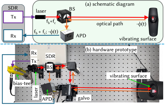
Fig. 3. Prototype overview. (a) We use a full-duplex SDR to simultaneously modulate the laser intensity and demodulate the photodetector output on the same board. The vibrating surface introduces a time-varying phase shift, \phi(t) , along the optical path, which the APD captures and the SDR extracts through the demodulation process in Fig. 2 (receiver). (b) Our hardware prototype shows the software-defined radio (SDR), laser, beam-splitter (BS), bias-tee, APD receiver, and vibrating surface used to close the sensing loop, all connected with standard RF cables.
