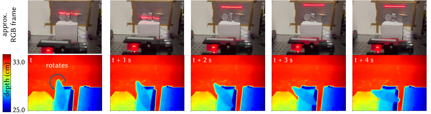
Fig. 11. Spatial depth scanning of dynamic scenes using a galvo system. A 250 \text{ px} \times 85 \text{ px} depth reconstruction of a rotating fan with static foreground objects (RGB shown for reference). Dense Lissajous scanning reconstructs the dynamic scene at 4 fps. The top row shows RGB frames from an approximate viewpoint corresponding to the depth scan, while the bottom row shows the reconstructed depth frames in cm. An illustration of the scanning process is provided in the supplementary material.
