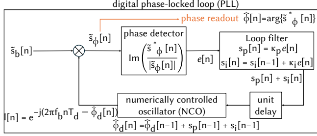
Fig. 14. Digital phase-locked loop (PLL) used for drift compensation. The downsampled baseband signal \tilde{s}_b[n] is mixed with a numerically controlled oscillator (NCO) to obtain the downconverted signal \tilde{s}_\phi[n] . A quadrature phase detector computes the phase error e[n] , which is filtered by a proportional–integral (PI) loop filter to update the NCO phase estimate \hat{\phi}_d[n] . The loop tracks slow oscillator drift while preserving higher-frequency phase variations corresponding to physical motion, which are obtained from the residual ToF phase \hat{\phi}[n] = \arg\{\tilde{s}_\phi^*[n]\} . The results are captured in Fig. 5 of the main paper.
