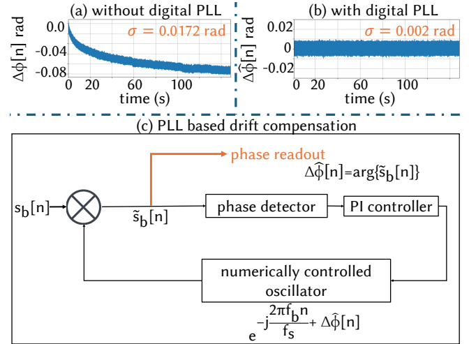
Fig. 5. Drift compensation using a digital phase-locked loop (PLL). (a) Raw phase measurements showing low-frequency drift in the SDR receiver. (b) Drift-compensated phase after applying the digital PLL, reducing phase standard deviation ( \sigma ) by approximately 10\times over a 140 s window. (c) Digital PLL schematic; the loop tracks slow oscillator drift while preserving higher-frequency phase variations from scene displacement.
