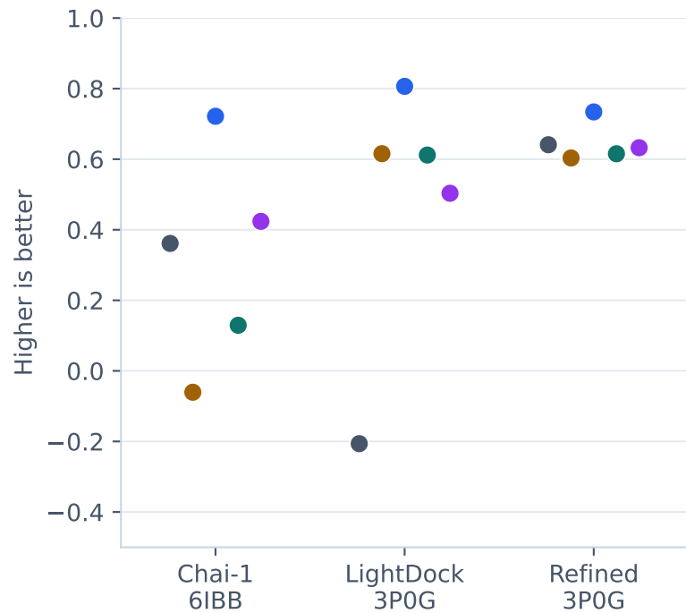
Rank correlation
