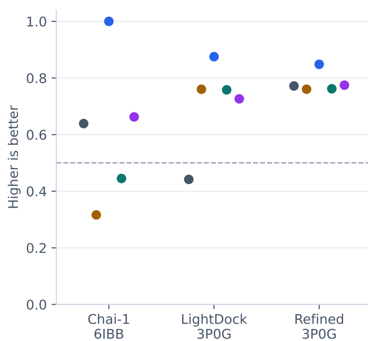
Correct-pose AUROC
