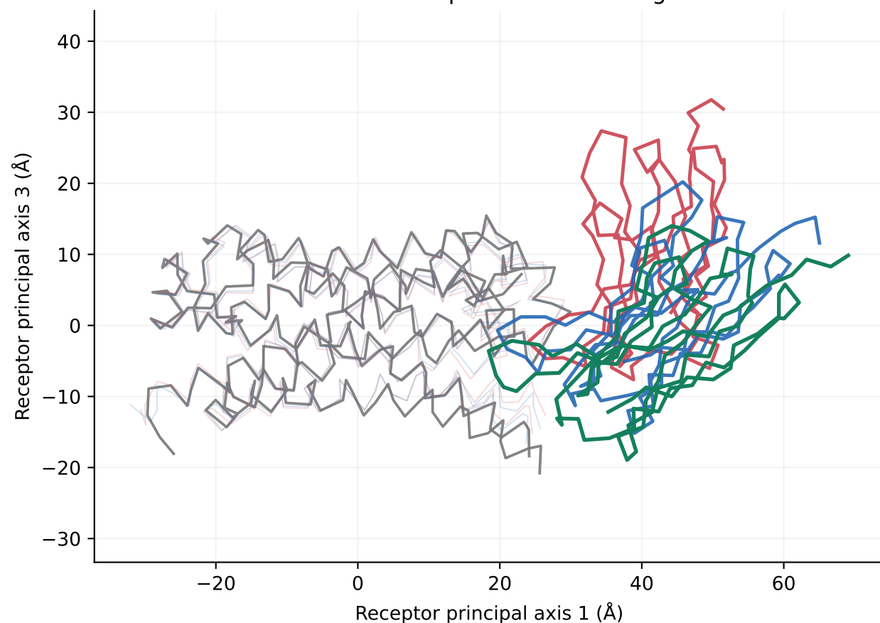
seed2_model_0 · full generated construct DockQ 0.485; ligand RMSD 6.90 Å
