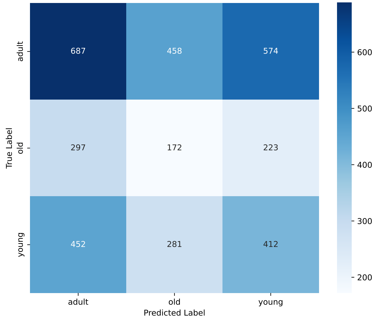
CNN — Confusion Matrix (Validation Set)
