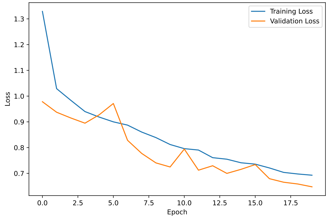
CNN — Loss
