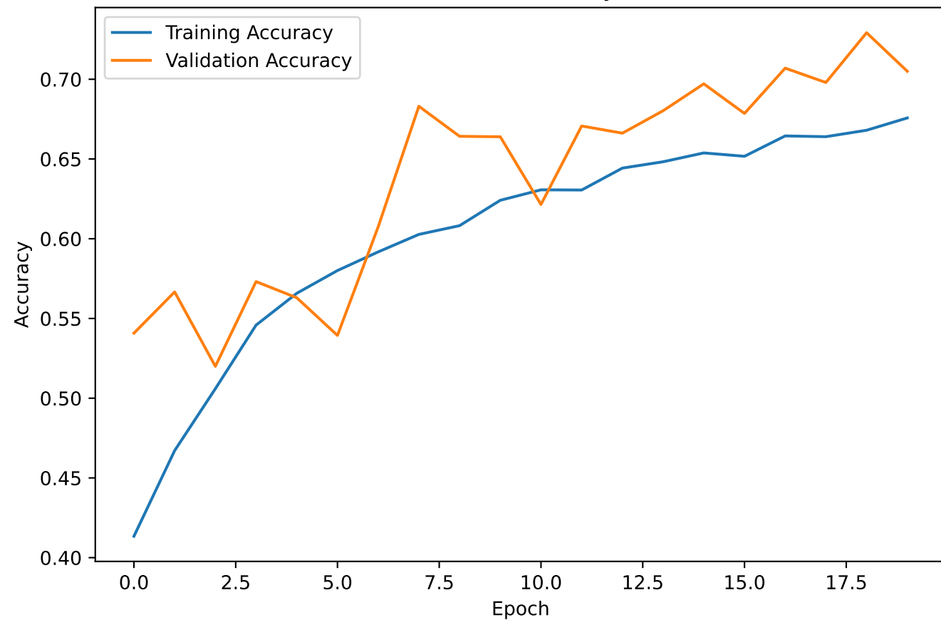
CNN — Accuracy
