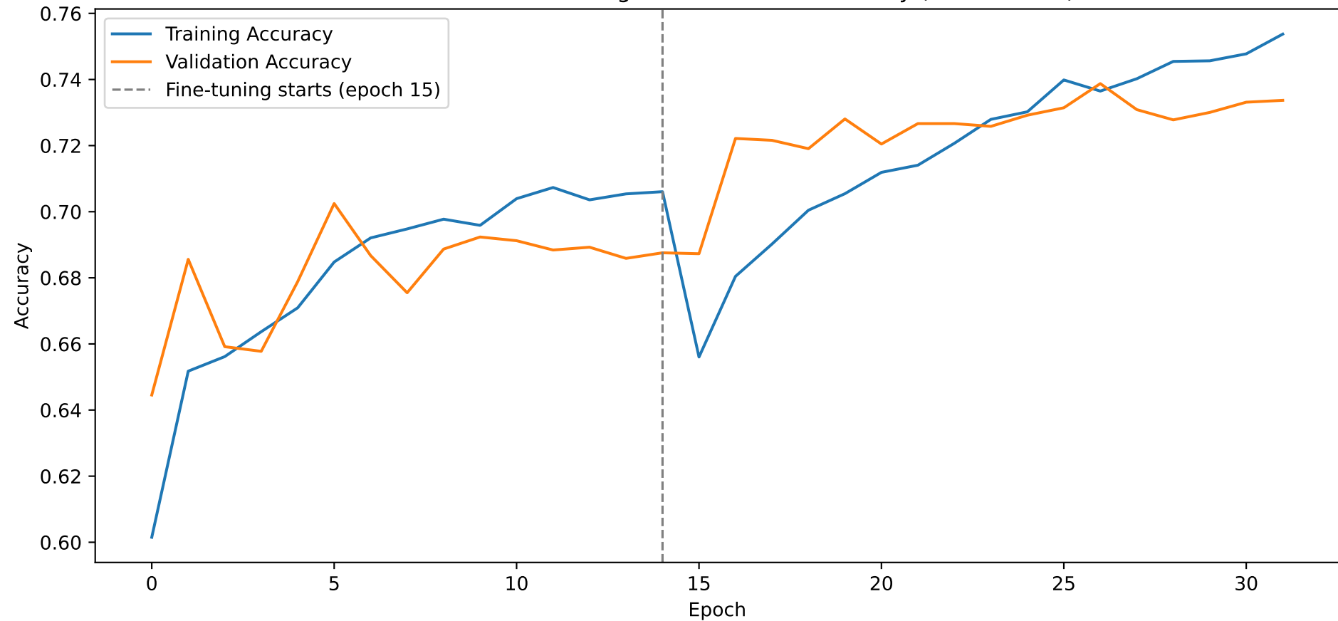
MobileNetV2 — Training and Validation Accuracy (Phase 1 + 2)
