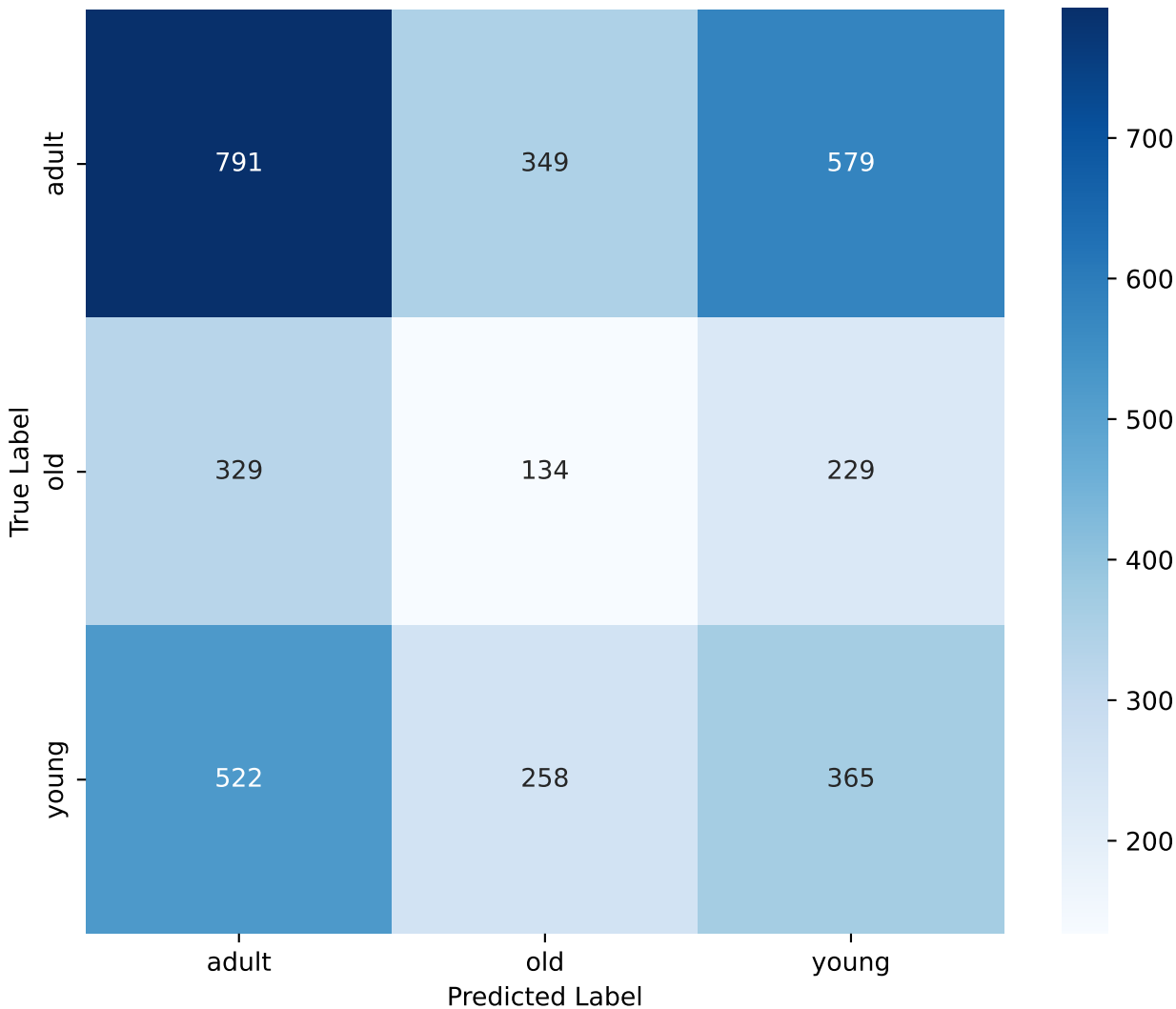
MobileNetV2 — Confusion Matrix (Validation Set)
