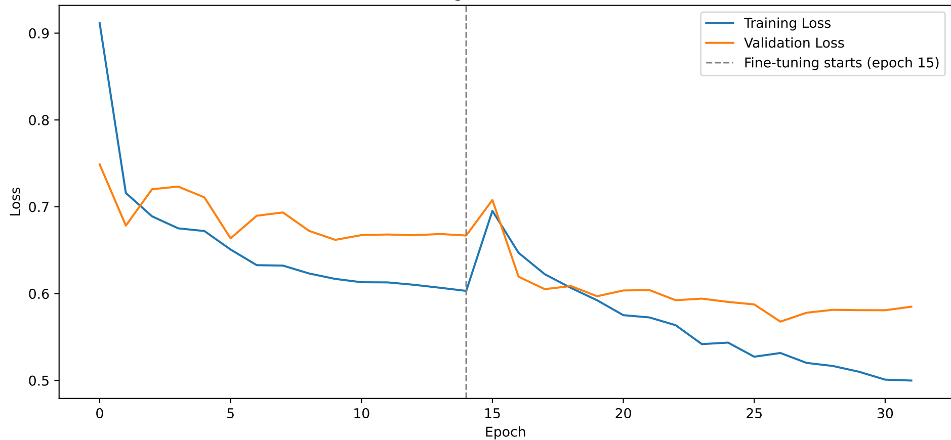
MobileNetV2 — Training and Validation Loss (Phase 1 + 2)
