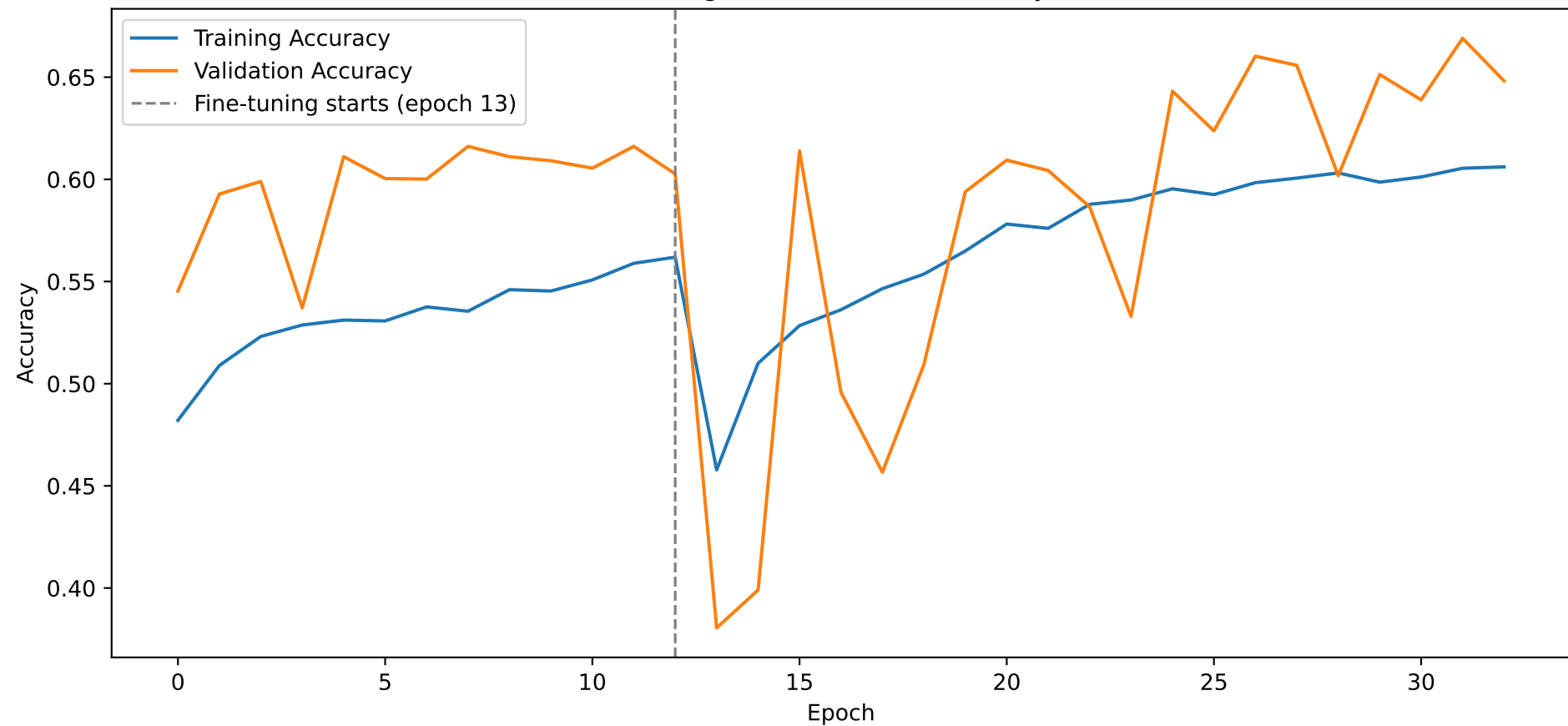
ResNet50 — Training and Validation Accuracy (Phase 1 + 2)
