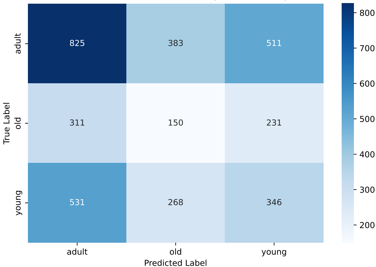
ResNet50 — Confusion Matrix (Validation Set)
