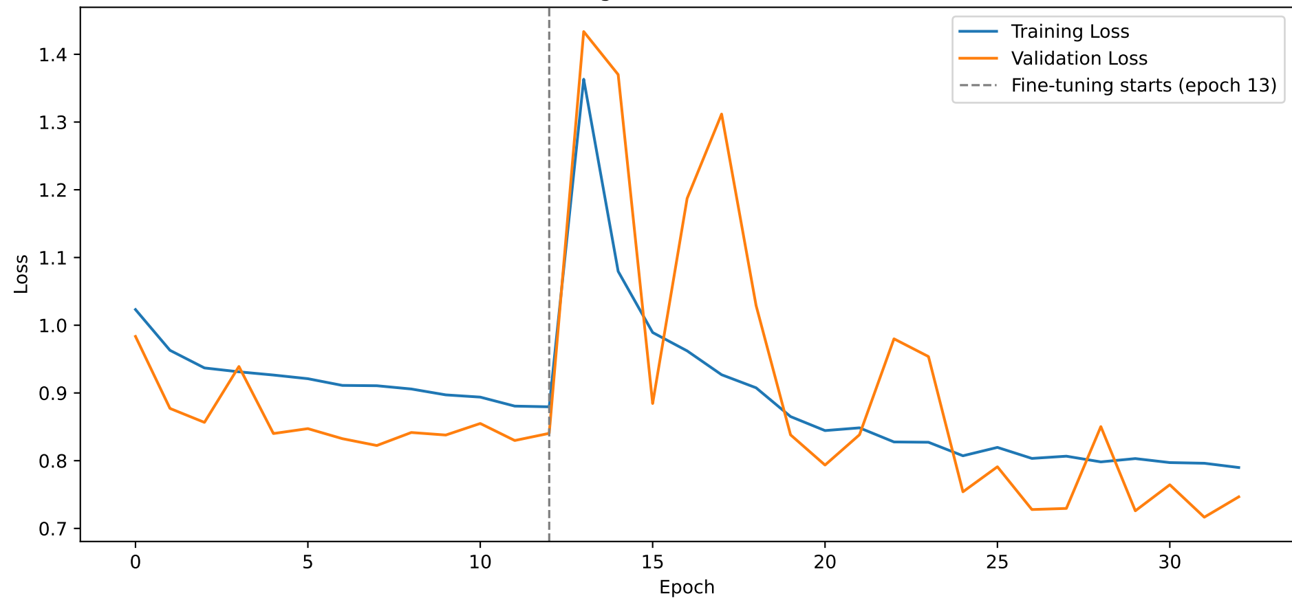
ResNet50 — Training and Validation Loss (Phase 1 + 2)
