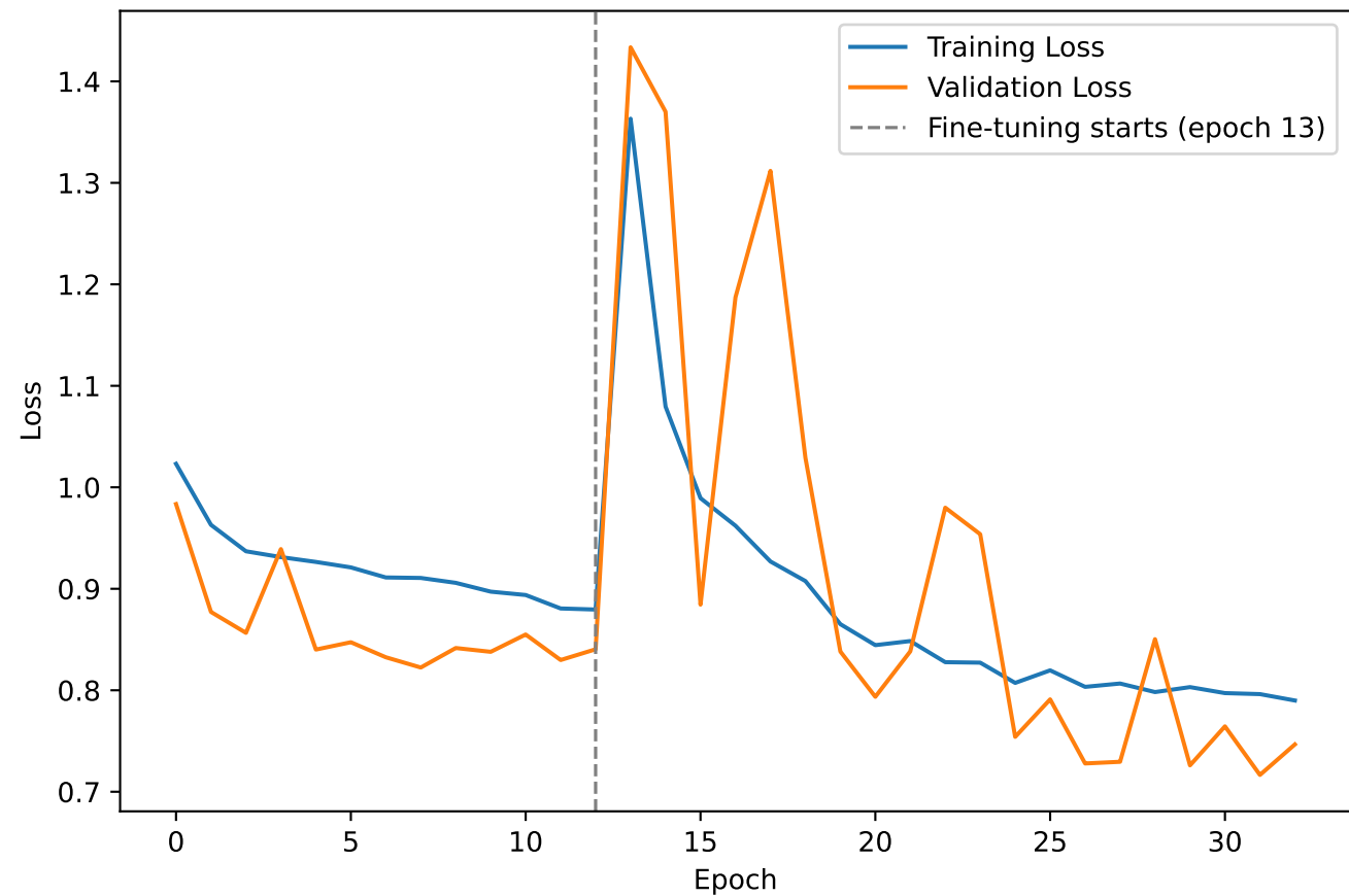
ResNet50 (Phase 1 + 2) — Loss
