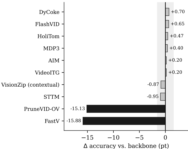
LLaVA-OV-7B (baseline 52.66%)
