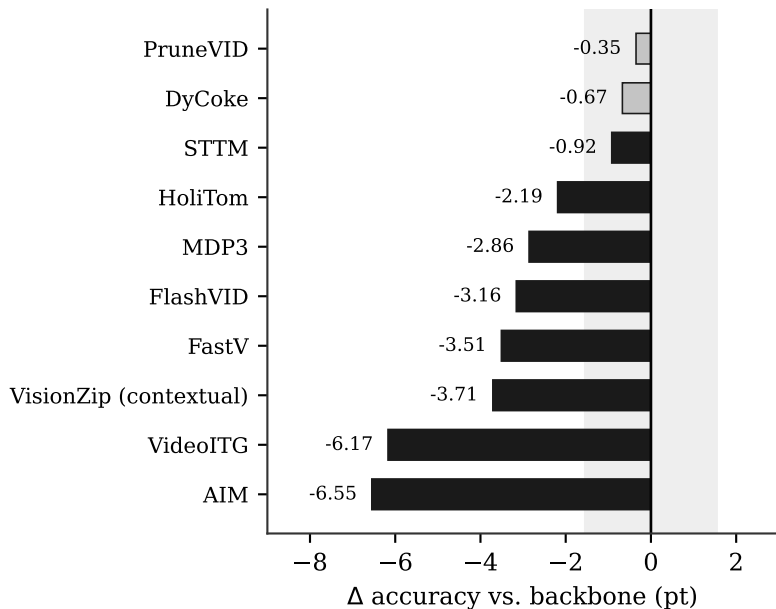
Qwen3-VL-8B (baseline 62.52%)
