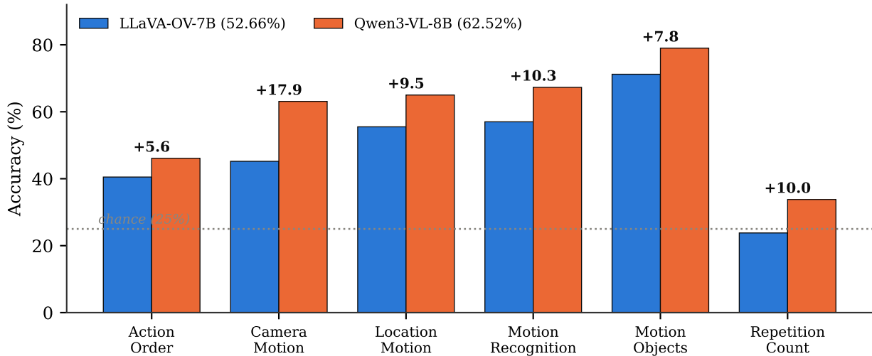
Baseline accuracy by question category
