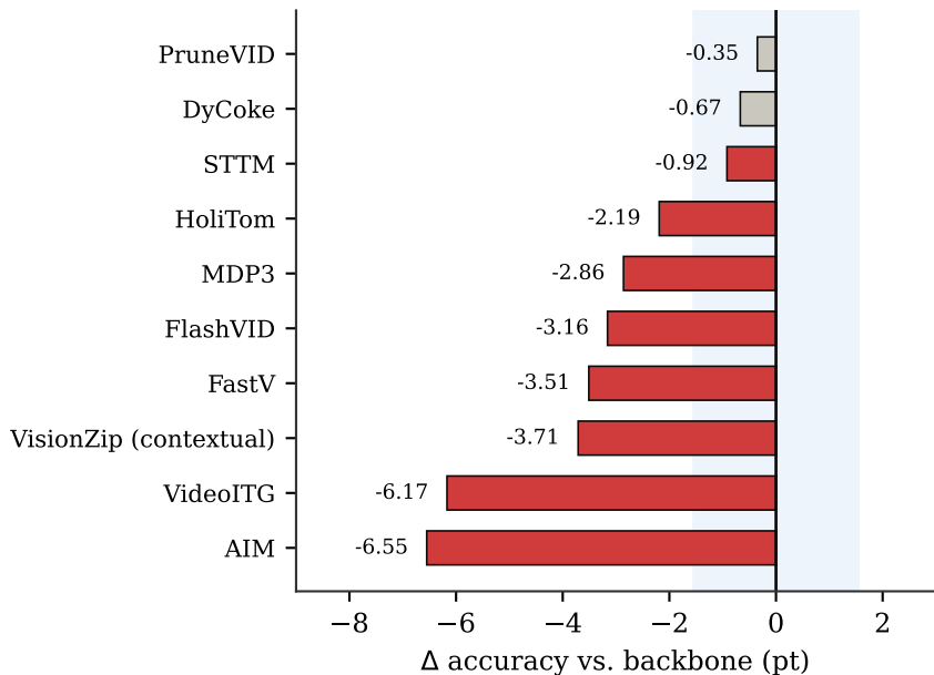
Qwen3-VL-8B (baseline 62.52%)
