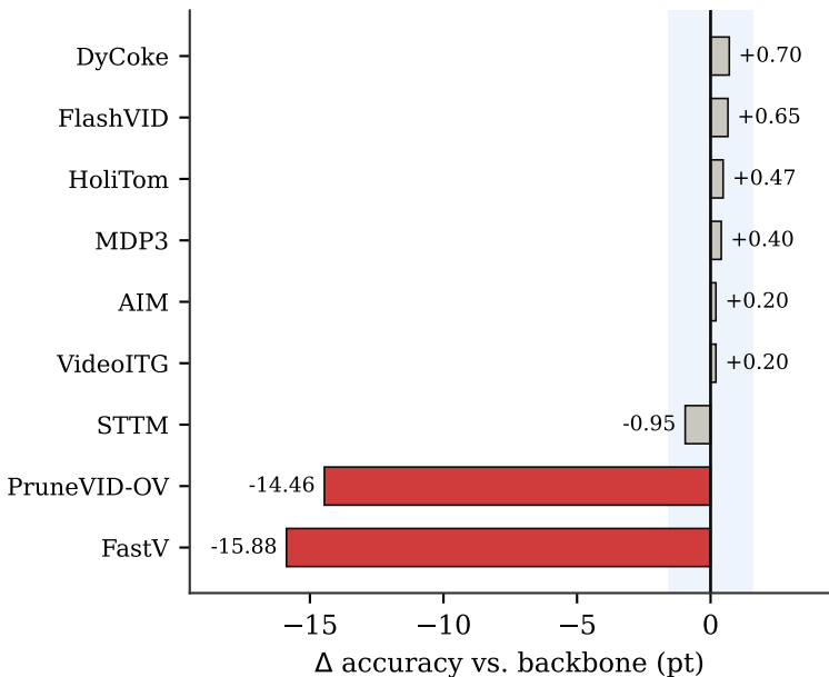
LLaVA-OV-7B (baseline 52.66%)
