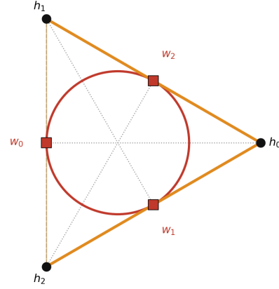
hinge h_0 's two legs (thick) graze at w_1, w_2 — never at its own w_0
