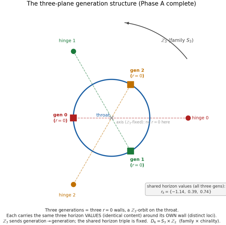
Figure 1: The three-plane fermion structure. Three hinges (radius 2\alpha , polar 0/120/240 ) and their three r = 0 walls (on the throat circle, polar 180/300/60 , each antipodal to its hinge)—a \mathbb{Z}_3 -orbit. Each plane carries the same three horizon values (identical content) around its own wall (distinct loci): three identical generations. The centre (the \mathbb{Z}_3 -fixed axis) carries no wall. \mathbb{Z}_3 sends generation to generation; D_6 = S_3 \times \mathbb{Z}_2 .
