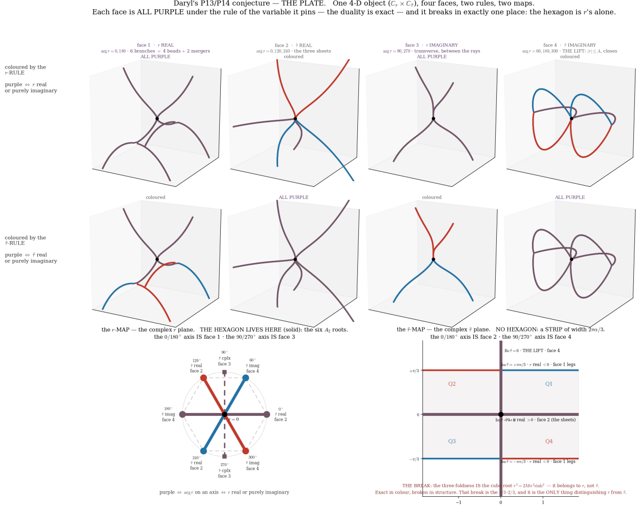
Figure 1: The Plate: the full analytic object \mathbb{C}_r \times \mathbb{C}_{\tilde{r}} on which the closure is stated (figure draft, to be finalised). The cosmogenetic bead r^3 = 2M\alpha^2 \sinh^2(3\tilde{r}/2\alpha) drawn as its four faces—the 2 \times 2 of \{r, \tilde{r}\} \times \{\text{real, imaginary}\} —under the two colouring rules and the two coordinate maps. The r -axis carries the A_2 hexagon, the discrete residue read as the three roots (the matter sector's flavour skeleton [20]); the \tilde{r} -axis carries the cosmogenetic lap, the two conjugate wings meeting at the branch point r = 0 . The mass-reflection R and the reality involution K of Proposition 3 are the two axis-symmetries of this one object, and the real slice (r, \tilde{r} \text{ real}) is the cosmological hyperboloid the framework paper draws panel by panel [7]. The conjugation of charge and the discrete residue of matter are thus one structure read two ways—Daryl's P13/P14 conjecture, carried here and drawn in full at the matter-sector seam.
