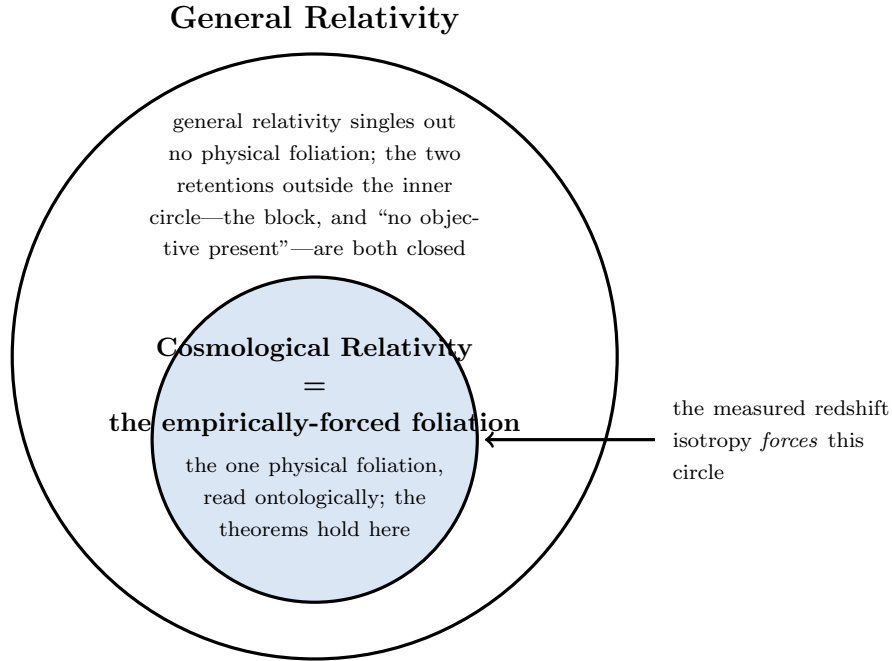
Figure 4: Cosmological Relativity as the necessary and sufficient augmentation of general relativity for a description of structural existence (Theorem ??). General relativity admits many foliations and singles out none; the augmentation fixes the one physical foliation and reads it ontologically, and by the redshift-isotropy forcing that foliation is measured rather than chosen [?] —so the augmented sub-region of general relativity and the empirically forced foliation are the same circle, and “CR” and “empirically-forced” are two names for it. The alternatives that would retain general relativity outside the circle are both closed: the block reading as a category error, “no objective present” as a modal fallacy falsified by the measured isotropy. Within the circle the programme’s theorems hold—the null–boundary correspondence, that collapsed matter must become a universe (Theorem ??), for gravitational collapse of any symmetry (Corollary ??).
