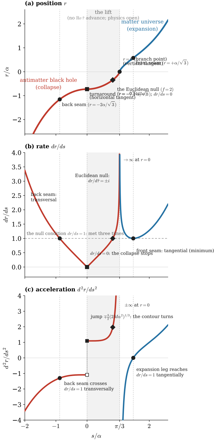
Figure 2: The lap in position, speed and acceleration , against the path length s along the bead's contour in complex cosmic time, on the Nariai member. Panel (a) is panel (F) of Fig. ??; (b) and (c) are its first and second derivatives, taken analytically on the same three closed-form segments (collapse, lift, expansion). Colour as throughout: red = antimatter ( r < 0 ), blue = matter ( r > 0 ); the shaded band is the lift, along which \text{Re } \tilde{\tau} does not advance. The dashed verticals mark the four loci. Their derivative signatures are all distinct (Remark ??), and the panels are to be read for the whole structure they carry, not only for the four marked loci. At the comoving turnaround the speed vanishes and the acceleration jumps sign through a finite corner, \mp \frac{3}{2}(2M\alpha^2)^{1/3} —the contour's right-angle turn. At r = 0 both diverge, the acceleration reversing sign; this is the areal coordinate degenerating rather than a dynamical turning. r = 0 is the branch point at the close of the lift, where the conjugate branch becomes the matter branch; the lap's seams are the two unit-speed loci r = -2\alpha/\sqrt{3} and r = +\alpha/\sqrt{3} . The organising feature of the lap is instead the null condition dr/ds = 1 , drawn as the dashed level in panel (b), and it is met three times. Both seams sit on it exactly : at the back seam r = -2\alpha/\sqrt{3} (where \cosh(3s/2\alpha) = 2 ) the collapse leg crosses it transversally , the acceleration finite and non-zero ( -1.299 ); at the front seam r = +\alpha/\sqrt{3} the expansion leg touches it tangentially , the speed attaining its minimum of exactly 1 and the acceleration vanishing. The two seams are therefore distinguished
