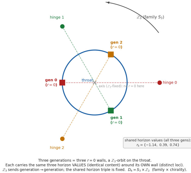
The three-plane generation structure (Phase A complete)
