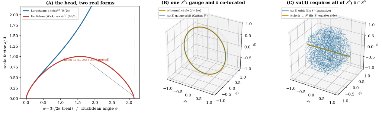
Figure 2: The QM Plate: the Euclidean real form, gauge and \hbar on one sphere (figure draft, to be finalised). The companion to Figure ?? on the substrate's other real form. (A) the bead's two real forms as one analytic curve—the Lorentzian \sinh^{2/3} (the open, temporal expansion) and its Euclidean Wick \sin^{2/3} , which closes at \beta = 2\pi\alpha , the horizon's thermal period. (B) the global-Wick S^5 = SO(6)/SO(5) carrying a \mathfrak{su}(3) gauge orbit (a Cartan torus) and the \hbar thermal great circle together, co-located on the one sphere. (C) a \mathfrak{su}(3) trajectory fills S^5 (the action is transitive) while the \hbar circle is a sub-orbit—the drawn form of \mathfrak{su}(3) \subset \mathfrak{so}(6) , \not\subset \mathfrak{so}(5) : gauge needs the whole sphere. All curves are integrated from the realified \mathfrak{su}(3) \subset \mathfrak{so}(6) generators (receipt R ); the projections of (B,C) are three-dimensional shadows of the five-sphere.
