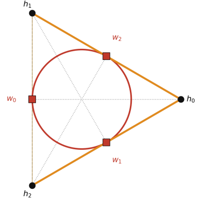
hinge h_0 's two legs (thick) graze at w_1, w_2 — never at its own w_0
