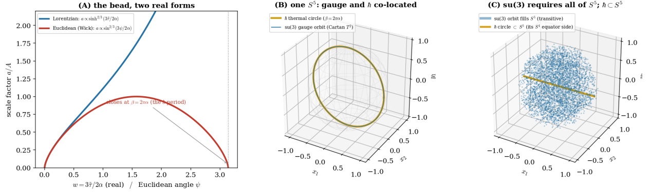
Figure 2: The QM Plate: the Euclidean real form, gauge and \hbar on one sphere. The companion to Figure 1 on the substrate's other real form. (A) the bead's two real forms as one analytic curve—the Lorentzian \sinh^{2/3} (the open, temporal expansion) and its Euclidean Wick \sin^{2/3} , which closes at \beta = 2\pi\alpha , the horizon's thermal period. (B) the global-Wick S^5 = SO(6)/SO(5) carrying a \mathfrak{su}(3) gauge orbit (a Cartan torus) and the \hbar thermal great circle together, co-located on the one sphere. (C) a \mathfrak{su}(3) trajectory fills S^5 (the action is transitive) while the \hbar circle is a sub-orbit—the drawn form of \mathfrak{su}(3) \subset \mathfrak{so}(6) , \not\subset \mathfrak{so}(5) : gauge needs the whole sphere. All curves are integrated from the realified \mathfrak{su}(3) \subset \mathfrak{so}(6) generators (receipt P13R11 ); the projections of (B,C) are three-dimensional shadows of the five-sphere.
