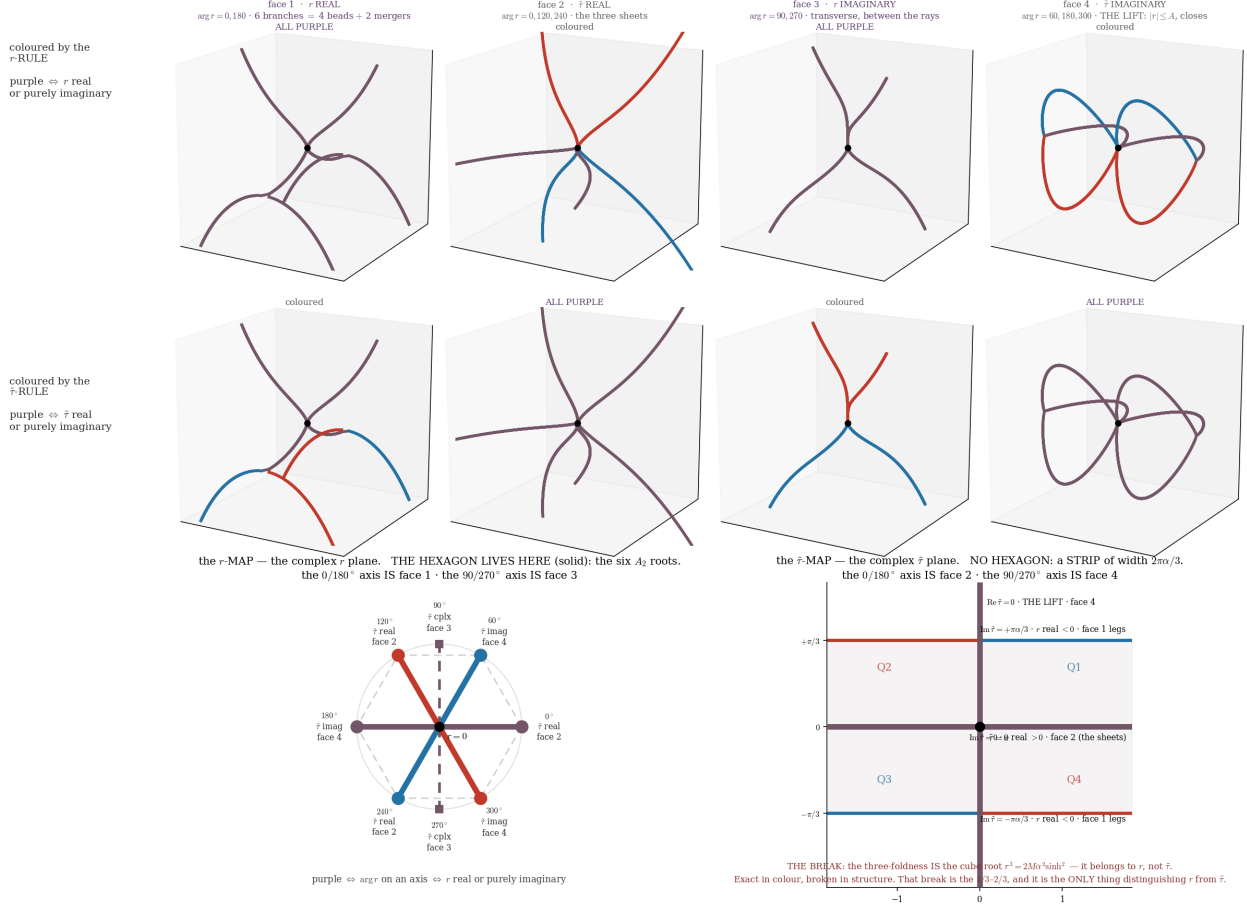
Figure 1: The Plate: the full analytic object \mathbb{C}_r \times \mathbb{C}_{\tilde{r}} on which the closure is stated The cosmogenetic bead r^3 = 2M\alpha^2 \sinh^2(3\tilde{r}/2\alpha) drawn as its four faces—the 2 \times 2 of \{r, \tilde{r}\} \times \{\text{real, imaginary}\} —under the two colouring rules and the two coordinate maps. The r -axis carries the A_2 hexagon, the discrete residue read as the three roots (the matter sector's flavour skeleton [20]); the \tilde{r} -axis carries the cosmogenetic lap, the two conjugate wings meeting at the branch point r = 0 . The mass-reflection R and the reality involution K of Proposition 3 are the two axis-symmetries of this one object, and the real slice (r, \tilde{r} \text{ real}) is the cosmological hyperboloid the framework paper draws panel by panel [7]. The conjugation of charge and the discrete residue of matter are thus one structure read two ways, drawn in full at the matter-sector seam.
