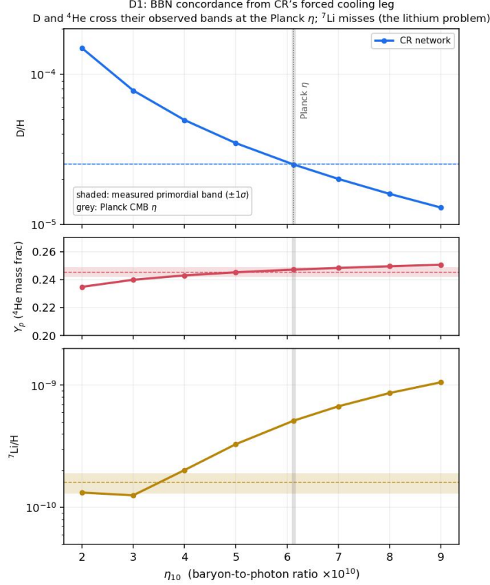
Figure 3: The BBN concordance from the computed cooling leg: light-element abundances against the baryon-to-photon ratio \eta (points, the network of Fig. 2 re-run across \eta ), with the measured primordial bands ( \pm 1\sigma , shaded) and the Planck CMB \eta (grey). Deuterium and helium-4 cross their observed bands at the CMB-fixed \eta ; lithium-7 lies above its band—the standard lithium problem, shared with flat \Lambda CDM.
