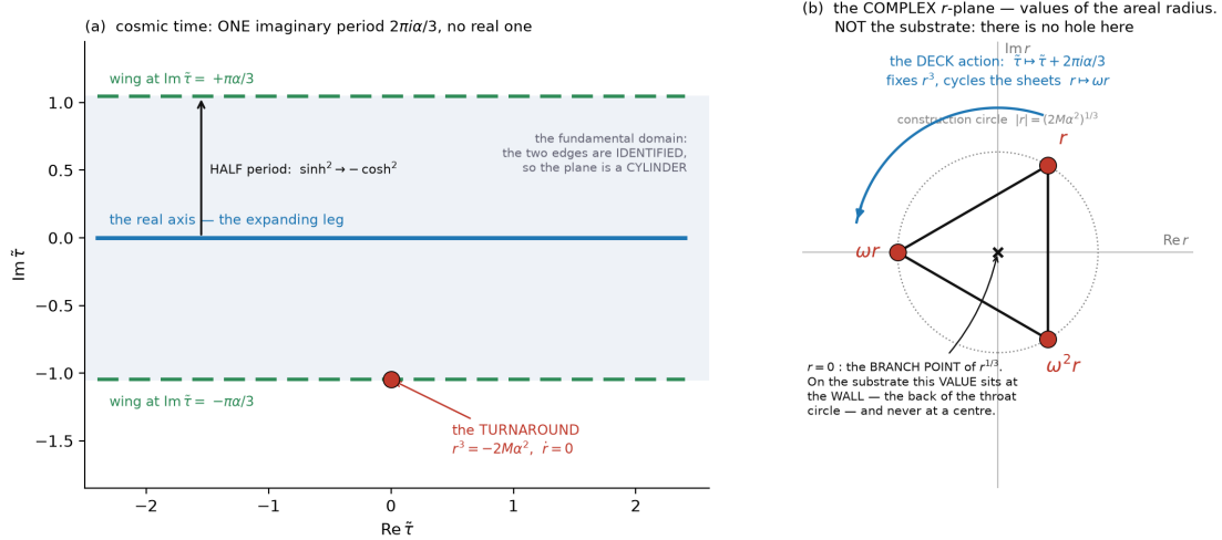
Figure 8: The construction's other three-ness, and the contrast with Figure 6 is the point of drawing it. P3R39 (a) The complexified cosmic-time plane of the bead's outward law r^3 = 2M\alpha^2 \sinh^2(3\tilde{\tau}/2\alpha) . That law has one imaginary period, 2\pi i\alpha/3 , and no real one, so the shaded band is a fundamental domain whose two edges are identified and the plane quotients to a cylinder—which is why everything here closes in elementary rather than elliptic terms. The half-period wings sit at \text{Im } \tilde{\tau} = \pm\pi\alpha/3 and carry \sinh^2 \mapsto -\cosh^2 , the real expanding leg to the conjugate collapse law; the turnaround is the point \tilde{\tau} = -i\pi\alpha/3 , where r^3 = -2M\alpha^2 and the velocity vanishes together, so it is a turnaround in fact and not by label. (b) The complex r -plane —a plane of values of the areal radius, and emphatically not a picture of the substrate, so that nothing in it is a hole and its centre is not a place. The three cube-root sheets the deck action \tilde{\tau} \mapsto \tilde{\tau} + 2\pi i\alpha/3 permutes: it leaves r^3 invariant and sends r \mapsto \omega r , and the three roots have one modulus with arguments spaced by exactly 120^\circ —equilateral, the dotted circle being a construction circle of radius (2M\alpha^2)^{1/3} recording that equality and nothing more. The origin deserves its own sentence, since it is the one point of this figure that is easily mislocated on the other. There r = 0 is the branch point of the cube root, a value ; on the substrate that value sits at the wall —the back of the throat circle, at X_1 = -\alpha , a point on the circle (§6.1)—and never at any centre, the interior of the throat carrying no manifold at all. The contrast with the hinge triple is total. That three indexes the within-state label, carries the full Weyl S_3 , lives in the equatorial section, and consists of roots of the horizon cubic at radius 2\alpha ; this one indexes the family [12], carries only the cyclic \mathbb{Z}_3 of the deck group, lives in complex cosmic time, and consists of sheets . The companion framework paper's lem:twoturnings establishes that no affine change of variable identifies the two root sets, so the two three-nesses are genuinely two, and reading a single figure as though it carried both is the error this pair of figures exists to prevent.
