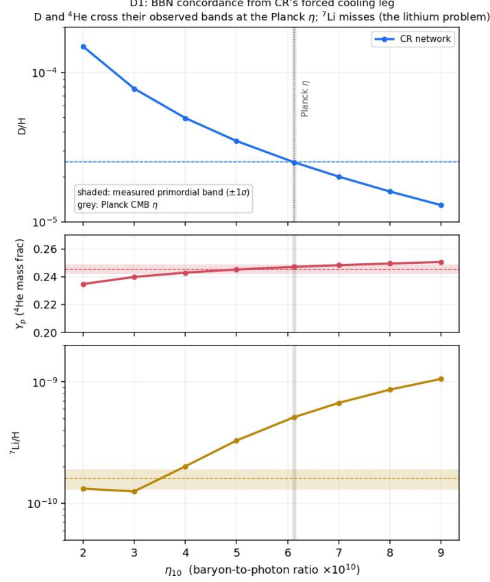
Figure 3: The BBN concordance from the computed cooling leg: light-element abundances against the baryon-to-photon ratio \eta (points, the network of Fig. ?? re-run across \eta ), with the measured primordial bands ( \pm 1\sigma , shaded) and the Planck CMB \eta (grey). Deuterium and helium-4 cross their observed bands at the CMB-fixed \eta ; lithium-7 lies above its band—the standard lithium problem, shared with flat \Lambda CDM.
