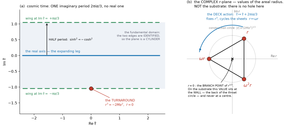
Figure 8: The construction's other three-ness, and the contrast with Figure 6 is the point of drawing it. P3R40 (a) The complexified cosmic-time plane of the bead's outward law r^3 = 2M\alpha^2 \sinh^2(3\tilde{\tau}/2\alpha) . That law has one imaginary period, 2\pi i\alpha/3 , and no real one, so the shaded band is a fundamental domain whose two edges are identified and the plane quotients to a cylinder—which is why everything here closes in elementary rather than elliptic terms. The half-period wings sit at \text{Im } \tilde{\tau} = \pm\pi\alpha/3 and carry \sinh^2 \mapsto -\cosh^2 , the real expanding leg to the conjugate collapse law; the turnaround is the point \tilde{\tau} = -i\pi\alpha/3 , where r^3 = -2M\alpha^2 and the velocity vanishes together, so it is a turnaround in fact and not by label. (b) The complex r -plane —a plane of values of the areal radius, and emphatically not a picture of the substrate, so that nothing in it is a hole and its centre is not a place. The three cube-root sheets the deck action \tilde{\tau} \mapsto \tilde{\tau} + 2\pi i\alpha/3 permutes: it leaves r^3 invariant and sends r \mapsto \omega r , and the three roots have one modulus with arguments spaced by exactly 120^\circ —equilateral, the dotted circle being a construction circle of radius (2M\alpha^2)^{1/3} recording that equality and nothing more. The origin deserves its own sentence, since it is the one point of this figure that is easily mislocated on the other. There r = 0 is the branch point of the cube root, a value ; on the substrate that value sits at the wall —the back of the throat circle, at X_1 = -\alpha , a point on the circle (§6.1)—and never at any centre, the interior of the throat carrying no manifold at all. The contrast with the hinge triple is total. That three indexes the within-state label, carries the full Weyl S_3 , lives in the equatorial section, and consists of roots of the horizon cubic at radius 2\alpha ; this one indexes the family [12], carries only the cyclic \mathbb{Z}_3 of the deck group, lives in complex cosmic time, and consists of sheets . The companion framework paper's lem:twoturnings establishes that no affine change of variable identifies the two root sets, so the two three-nesses are genuinely two, and reading a single figure as though it carried both is the error this pair of figures exists to prevent.
