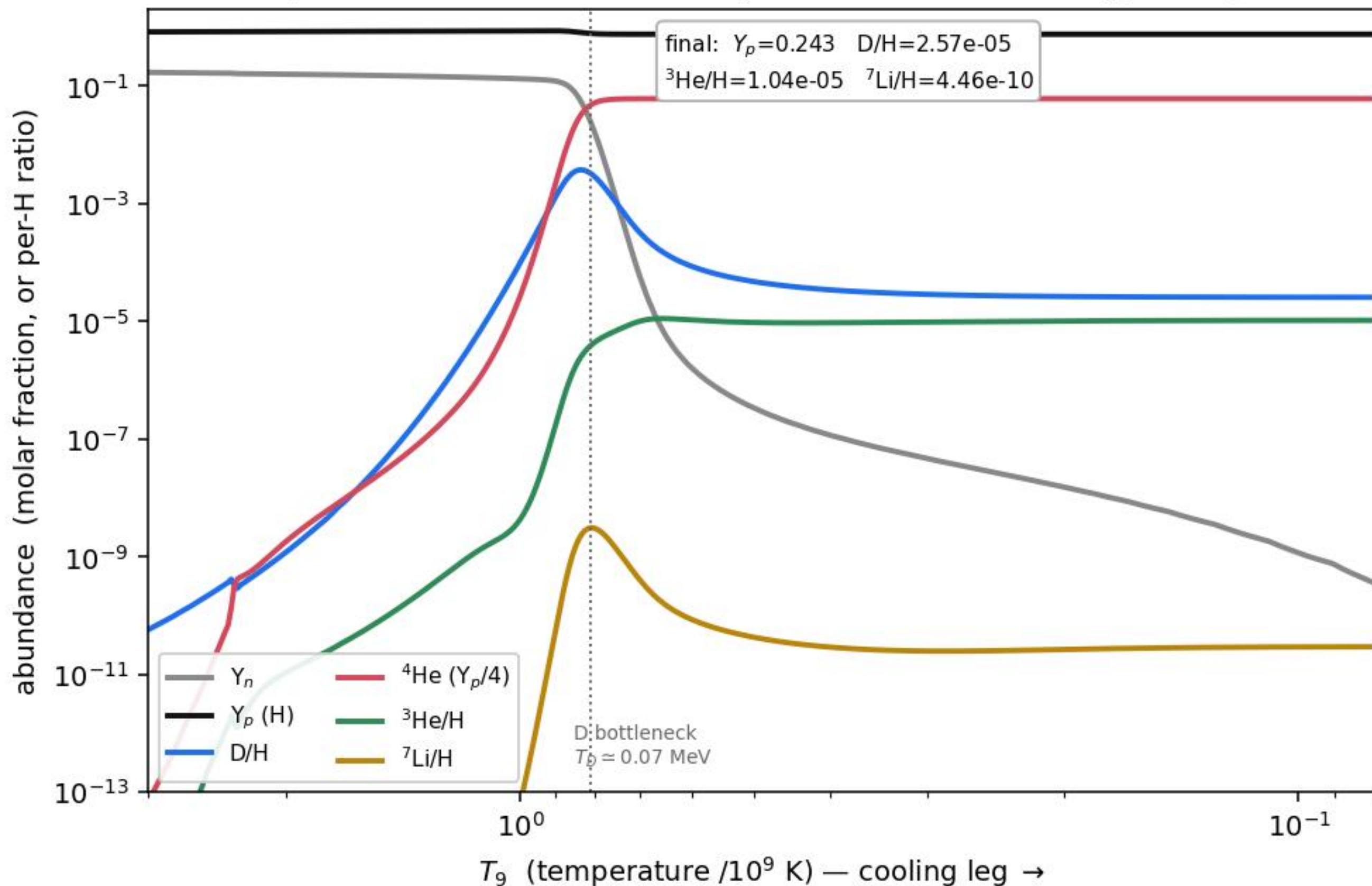
D1: light elements freezing out on the collapse cooling leg (REACLIB network + thermal n \leftrightarrow p , standard window rate, \eta_{10} = 6.14 )
