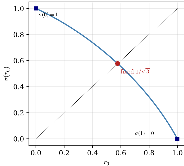
(b) root-exchange involution \sigma
