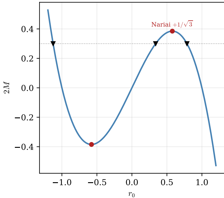
(a) horizon cubic 2M = r_0 - r_0^3
