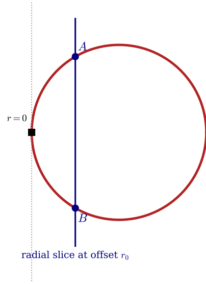
(b) equator-on: the throat circle
