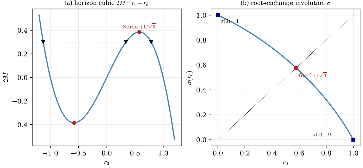
Figure 2: (a) The horizon cubic in the form 2M = r_0 - r_0^3 . A given value of 2M is met by three roots (three horizons); the triplet is the content of the factorisation (??). The marked extrema at r_0 = \pm 1/\sqrt{3} are the Nariai double-root locus. (b) The root-exchange involution \sigma(r_0) = \frac{1}{2}(-r_0 + \sqrt{4 - 3r_0^2}) , with \sigma(\sigma(r_0)) = r_0 . It exchanges the endpoints 0 \leftrightarrow 1 and fixes r_0 = 1/\sqrt{3} , the Nariai configuration.
