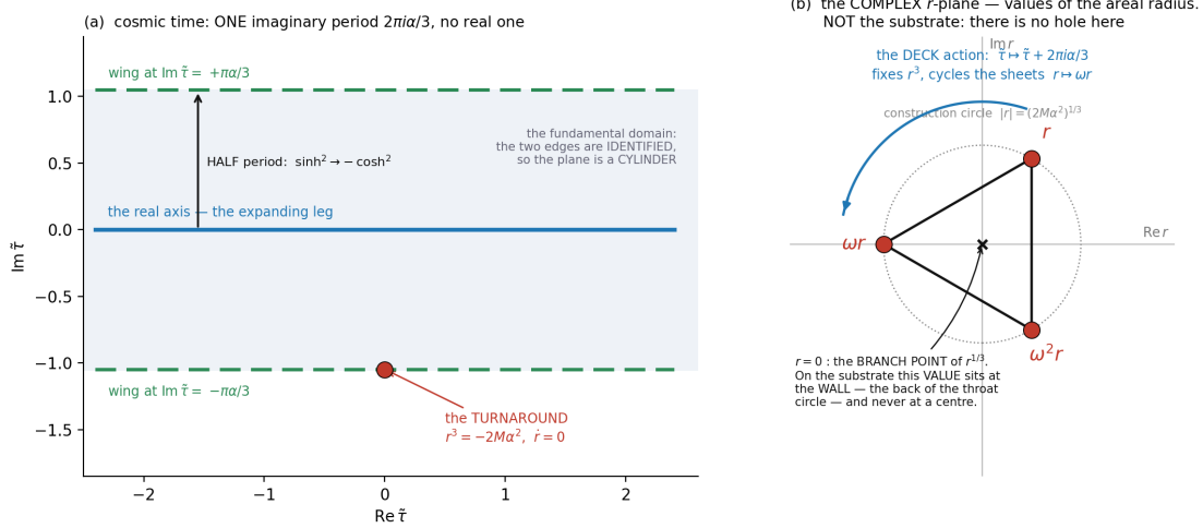
Figure 8: The construction's other three-ness, and the contrast with Figure ?? is the point of drawing it. R (a) The complexified cosmic-time plane of the bead's outward law r^3 = 2M\alpha^2 \sinh^2(3\tilde{\tau}/2\alpha) . That law has one imaginary period, 2\pi i \alpha/3 , and no real one, so the shaded band is a fundamental domain whose two edges are identified and the plane quotients to a cylinder—which is why everything here closes in elementary rather than elliptic terms. The half-period wings sit at \text{Im } \tilde{\tau} = \pm\pi\alpha/3 and carry \sinh^2 \mapsto -\cosh^2 , the real expanding leg to the conjugate collapse law; the turnaround is the point \tilde{\tau} = -i\pi\alpha/3 , where r^3 = -2M\alpha^2 and the velocity vanishes together, so it is a turnaround in fact and not by label. (b) The complex r -plane —a plane of values of the areal radius, and emphatically not a picture of the substrate, so that nothing in it is a hole and its centre is not a place. The three cube-root sheets the deck action \tilde{\tau} \mapsto \tilde{\tau} + 2\pi i \alpha/3 permutes: it leaves r^3 invariant and sends r \mapsto \omega r , and the three roots have one modulus with arguments spaced by exactly 120^\circ —equilateral, the dotted circle being a construction circle of radius (2M\alpha^2)^{1/3} recording that equality and nothing more. The origin deserves its own sentence, since it is the one point of this figure that is easily mislocated on the other. There r = 0 is the branch point of the cube root, a value ; on the substrate that value sits at the wall —the back of the throat circle, at X_1 = -\alpha , a point on the circle (§??)—and never at any centre, the interior of the throat carrying no manifold at all. The contrast with the hinge triple is total. That three indexes the within-state label, carries the full Weyl S_3 , lives in the equatorial section, and consists of roots of the horizon cubic at radius 2\alpha ; this one indexes the family [?], carries only the cyclic \mathbb{Z}_3 of the deck group, lives in complex cosmic time, and consists of sheets . The companion framework paper's lem:twoturnings establishes that no affine change of variable identifies the two root sets, so the two three-nesses are genuinely two, and reading a single figure as though it carried both is the error this pair of figures exists to prevent.
