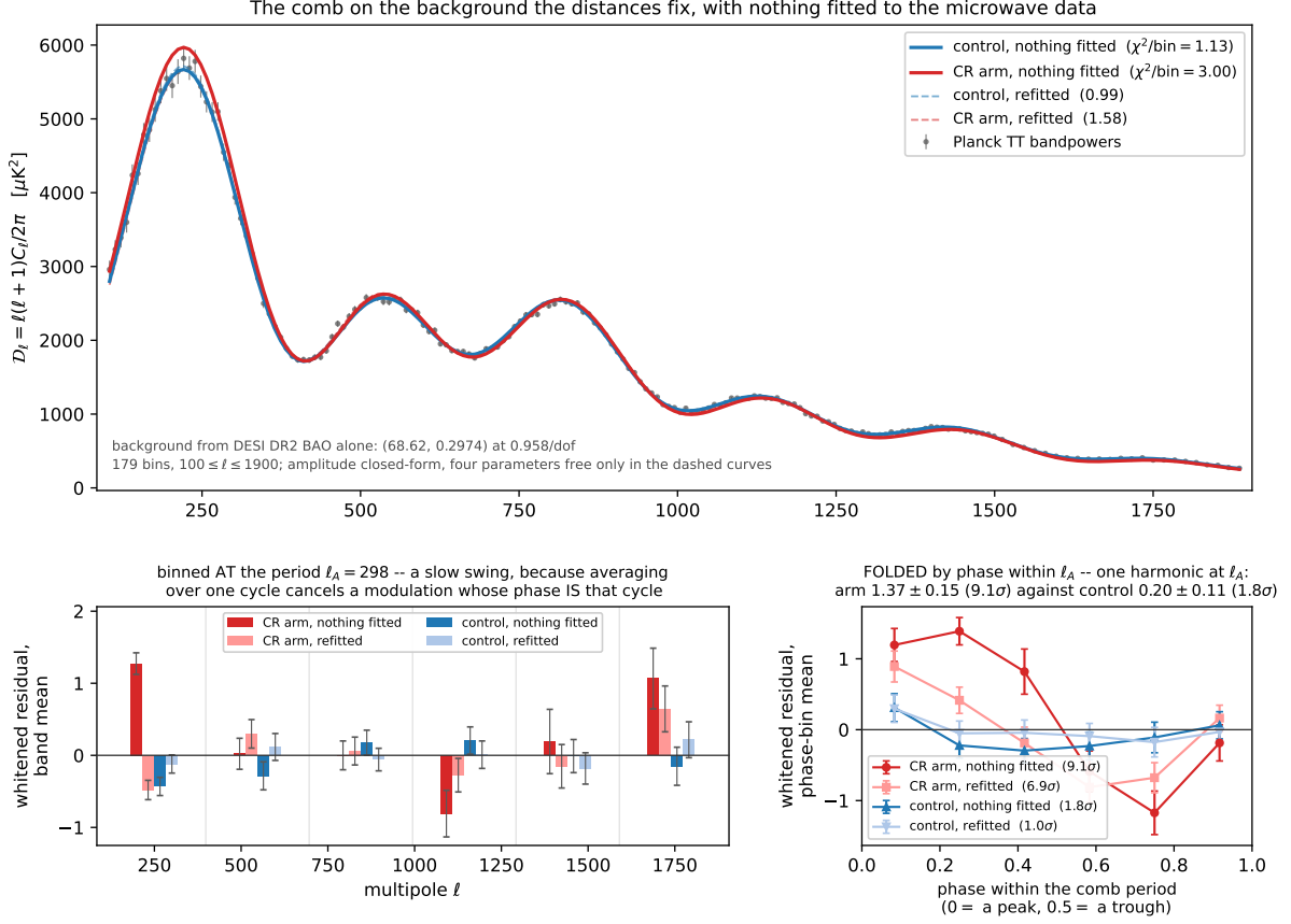
Figure 3: The other confrontation: the comb computed on the background the distance data fix, with nothing fitted to the microwave data. Above , both arms in D_\ell against the Planck temperature bandpowers, on a background recovered from DESI DR2 baryon-acoustic data alone—(68.62, 0.2974) at 0.958 per degree of freedom P15R163P15R236 —with the overall amplitude in closed form and no other number taken from the spectrum; the dashed curves are the refit minima of Fig. 2 for comparison on the same bins. Over 179 bins on 100 \leq \ell \leq 1900 the control stands at 1.13 per bin and this arm at 3.00, a factor 2.66, against 0.99 and 1.58 when four parameters are freed in each arm. The peaks are the thing to look at: positions and spacing agree while the extrema are overshoot, which is the rejection in the form a reader can see. Below left , the whitenened residual averaged in bins one comb period wide. It shows a slow swing changing sign twice across the range and no alternation—and it cannot show one, because averaging over a full cycle of a modulation at that period returns that modulation’s own mean. The panel is drawn because the operation is the one a reader reaches for, and what it does show is a true and separate statement about the residual’s long-wavelength shape. Below right , the measurement: the same residual folded by phase within the comb period, anchored on this arm’s own first peak. One harmonic at \ell_A has amplitude 1.37 \pm 0.15 for the unfitted arm— 9.1\sigma —against the control’s 0.20 \pm 0.11 , consistent with none; freeing the four parameters halves it to 0.81 \pm 0.12 and leaves 6.9\sigma . So the rejection is shaped at the acoustic period, the shape survives the refit, and the free parameters absorb part of it without reaching its cause. P15R279
