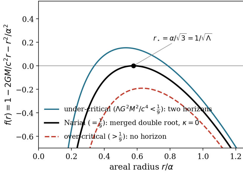
Figure 4: The Schwarzschild–de Sitter metric function f(r) = 1 - 2GM/c^2 r - r^2/\alpha^2 across the three regimes. Under-critical masses ( \Lambda G^2 M^2 / c^4 < \frac{1}{9} ) give two distinct positive horizons; over-critical masses give none. The cosmogenesis branch point is carried on the Nariai member ( = \frac{1}{9} ), where the two horizons merge into a single degenerate double root at r_N = \alpha/\sqrt{3} = 1/\sqrt{\Lambda} with f(r_N) = f'(r_N) = 0 and hence vanishing surface gravity \kappa = 0 . The degeneracy of this root is what the throat geometry (Proposition 4) and the transmission dichotomy (§8) turn on.
