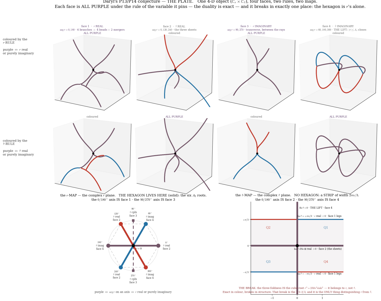
Figure 1: The Plate: the full analytic object \mathbb{C}_r \times \mathbb{C}_{\tilde{r}} on which the closure is stated The cosmogenetic bead r^3 = 2M\alpha^2 \sinh^2(3\tilde{r}/2\alpha) drawn as its four faces—the 2 \times 2 of \{r, \tilde{r}\} \times \{\text{real}, \text{imaginary}\} —under the two colouring rules and the two coordinate maps. The r -axis carries the A_2 hexagon, the discrete residue read as the three roots (the matter sector's three seats [20]); the \tilde{r} -axis carries the cosmogenetic lap, the two conjugate wings meeting at the branch point r = 0 . The mass-reflection R and the reality involution K of Proposition 3 are the two axis-symmetries of this one object, and the real slice (r, \tilde{r} \text{ real}) is the cosmological hyperboloid the framework paper draws panel by panel [7]. The conjugation of charge and the discrete residue of matter are thus one structure read two ways, drawn in full at the matter-sector seam.
