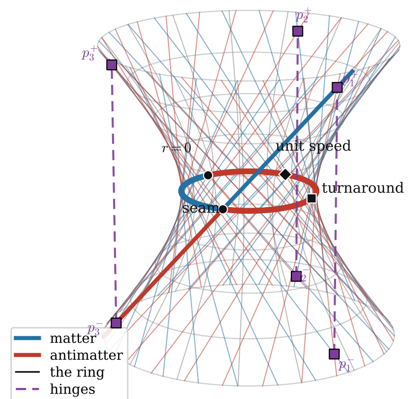
(B) the dS_4 background
