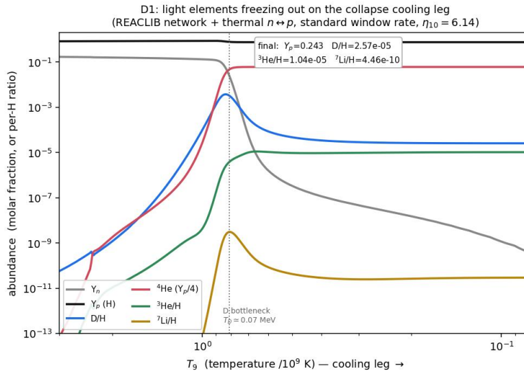
Figure 2: The light elements freezing out along the expanding leg, computed by a genuine multi-nuclide network (published REACLIB rates, forward and detailed-balance reverse, with the finite-temperature weak n \leftrightarrow p conversion) integrated on the standard window rate of Sec 4 at the inherited \eta_{10} = 6.14 . Deuterium rises through the bottleneck T_D (dotted) and burns down to its relic; helium-4 plateaus; lithium-7 and helium-3 settle at their standard values. The pattern reproduces standard big-bang nucleosynthesis to a few percent, with the correct \eta -dependence and baryon number conserved through the integration.
