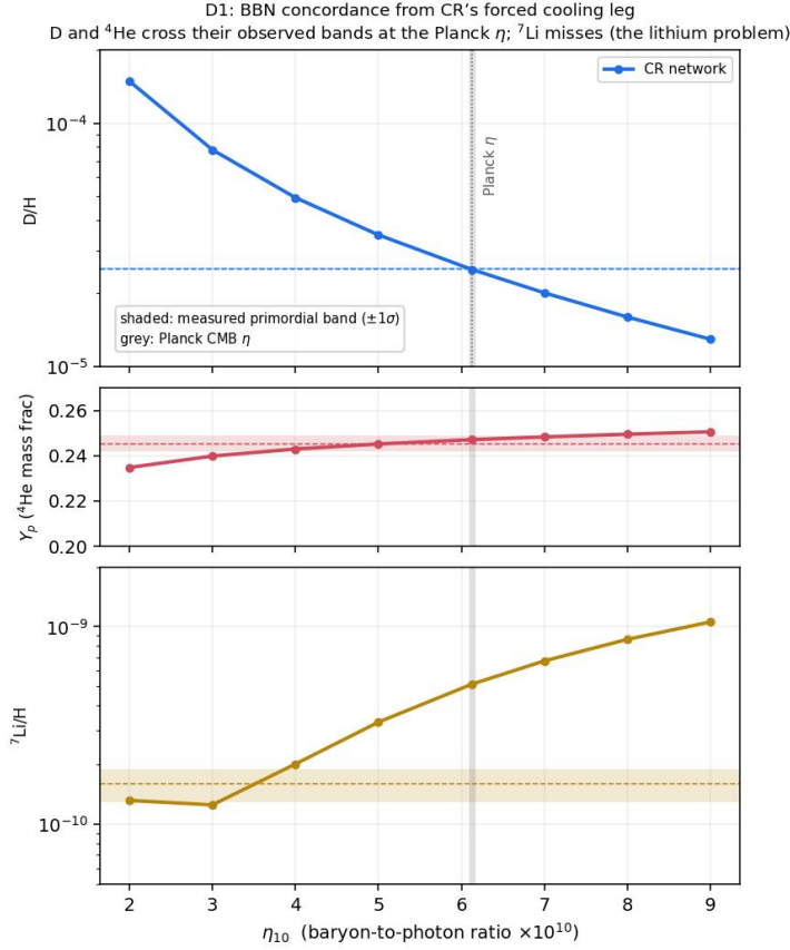
Figure 3: The BBN concordance from the computed cooling leg: light-element abundances against the baryon-to-photon ratio \eta (points, the network of Fig. ?? re-run across \eta ), with the measured primordial bands ( \pm 1\sigma , shaded) and the Planck CMB \eta (grey). Deuterium and helium-4 cross their observed bands at the CMB-fixed \eta ; lithium-7 lies above its band—the standard lithium problem, shared with flat \Lambda CDM.
