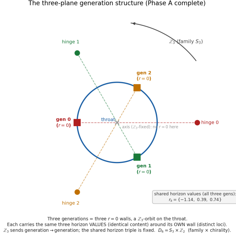
Figure 1: The three-plane fermion structure. Three hinges (radius 2\alpha , polar 0/120/240) and their three r=0 walls (on the throat circle, polar 180/300/60, each antipodal to its hinge)—a \mathbb{Z}_3 -orbit. Each plane carries the same three horizon values (identical content) around its own wall (distinct loci): three identical bound modes, whose number is what the wall structure fixes (§6.1). The centre (the \mathbb{Z}_3 -fixed axis) carries no wall. \mathbb{Z}_3 sends wall to wall; D_6 = S_3 \times \mathbb{Z}_2 .
