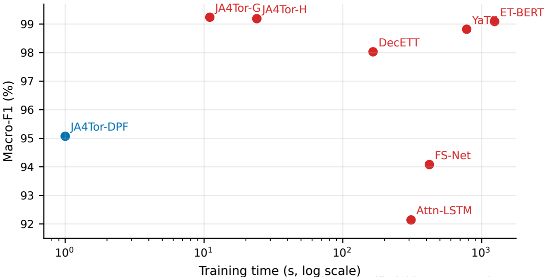
Accuracy-cost positioning
