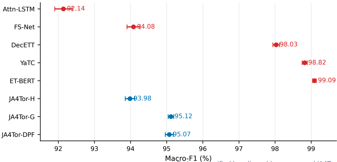
Pcap-disjoint five-class comparison
