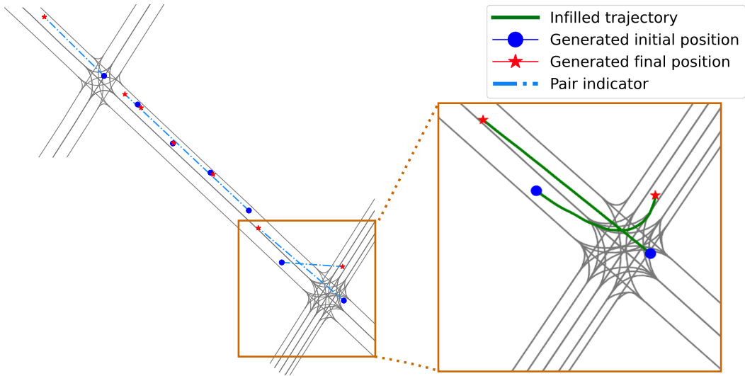
(a) High-level traffic scenario
