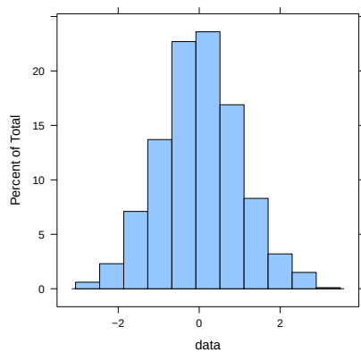
(a) Histogram
