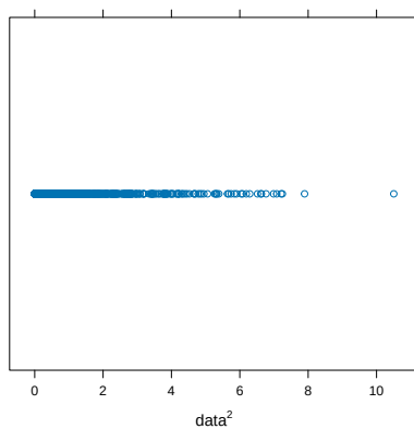
(c) Stripplot
