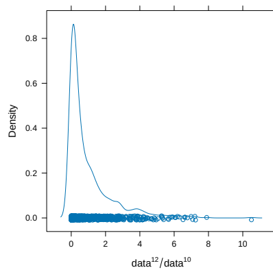
(b) Densityplot
