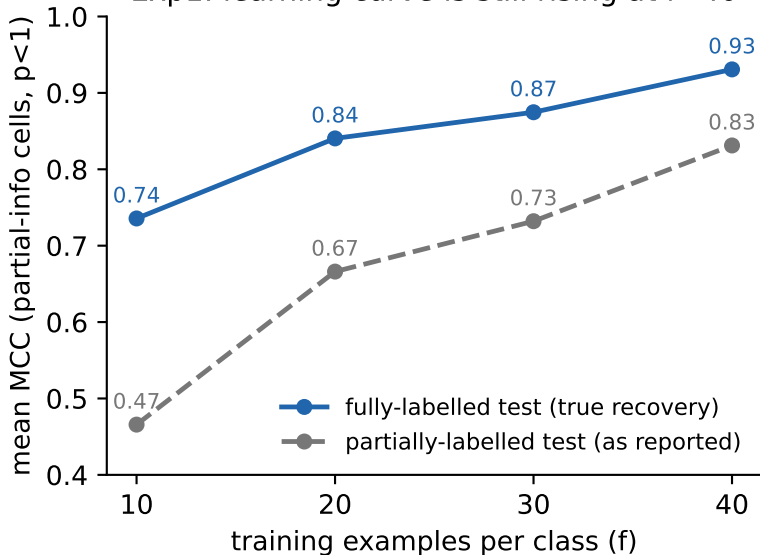
Exp1: learning curve is still rising at f=40
