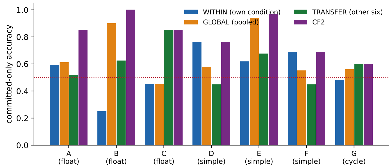
Exp2: contextual-reasoning test — one pooled semantics beats seven specialised ones
