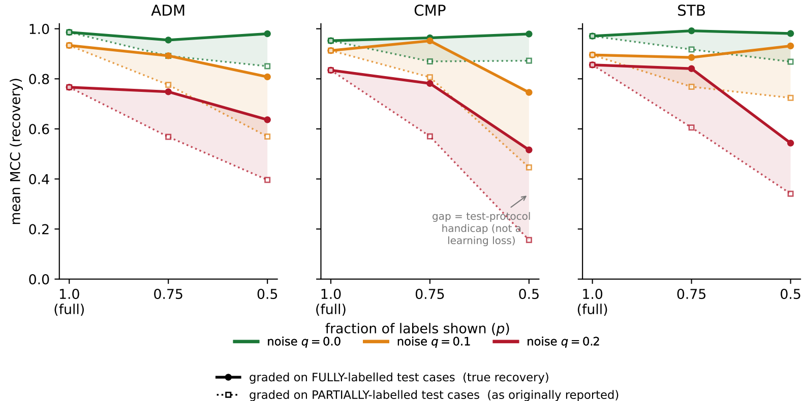
Exp1: how well the learner recovers the target semantics (same learned theories, scored two ways)
