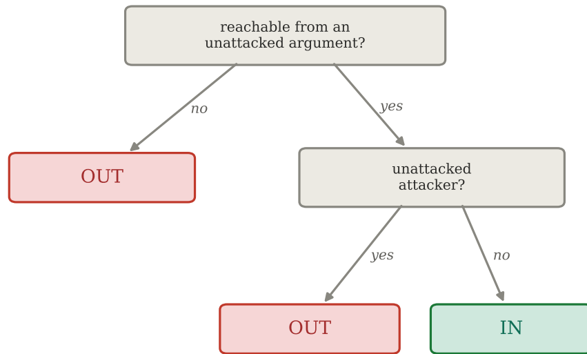
(a) grounded — 3 clean rules (MCC 0.86)
