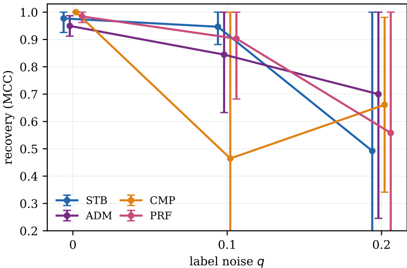
Partial labels ( p = 0.5 ), f = 20 balanced
